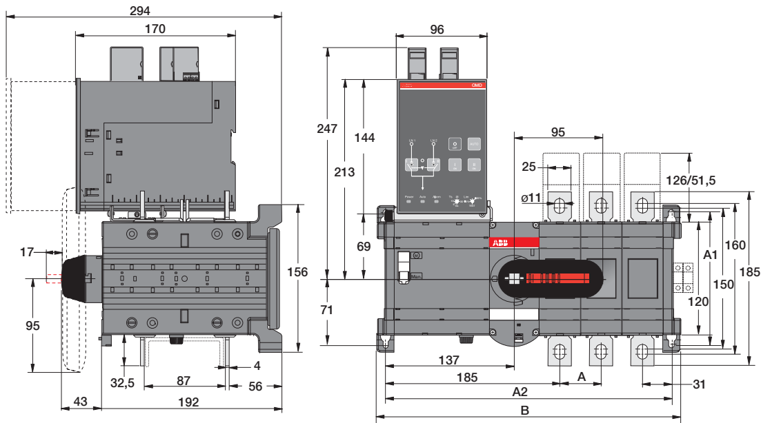
OTM315...400E_C_2D_, OTM315...400E_C_3D
