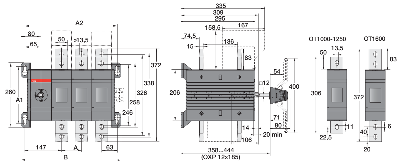
OT1000...1600E03/04CP
