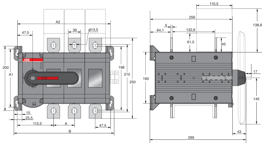
OT630...800E03/04C with direct mount handle
