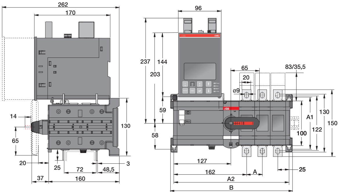
OTM160...250E_C_8D_
