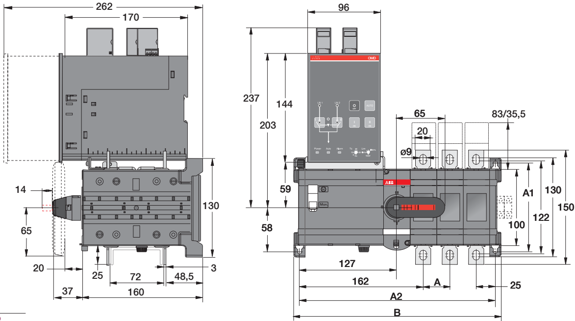
OTM160...250E_C_2D_, OTM160...250E_C_3D_
