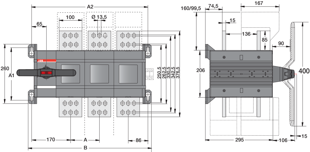
OT2000...2500E03/04C with direct mount handle
