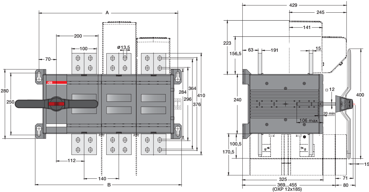
OT3200E03/04CP
