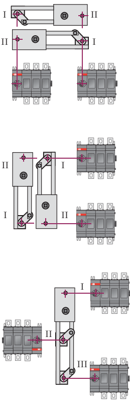
Change-over and by-pass switches
