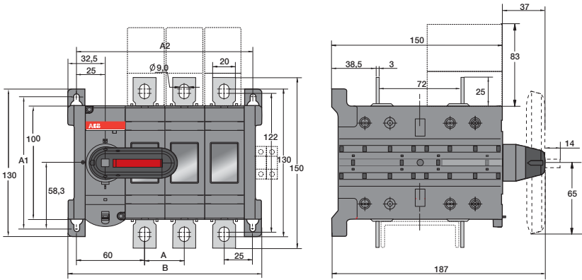
OT160...250E03/04C with direct mount handle
